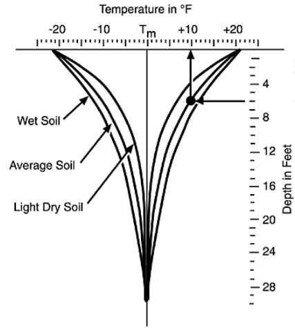
Figure 5. Soil Temperature Variations by Depth (Department of Energy, 1994)
